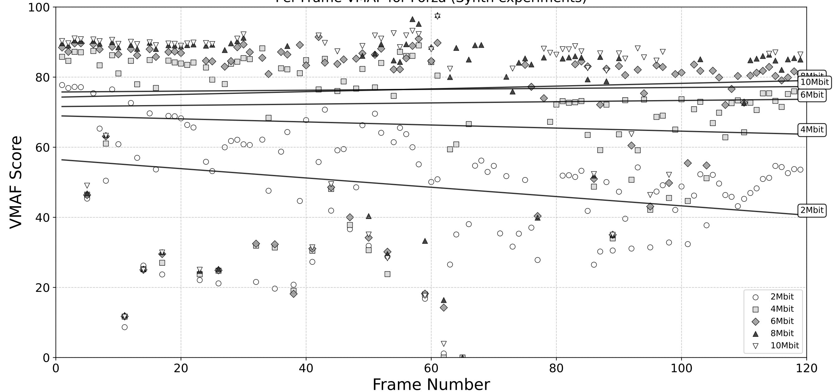
Per-Frame VMAF for Forza (Synth experiments)
