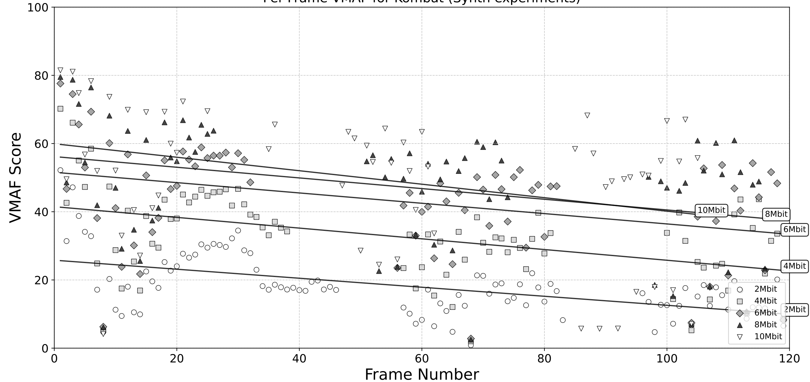
Per-Frame VMAF for Kombat (Synth experiments)
