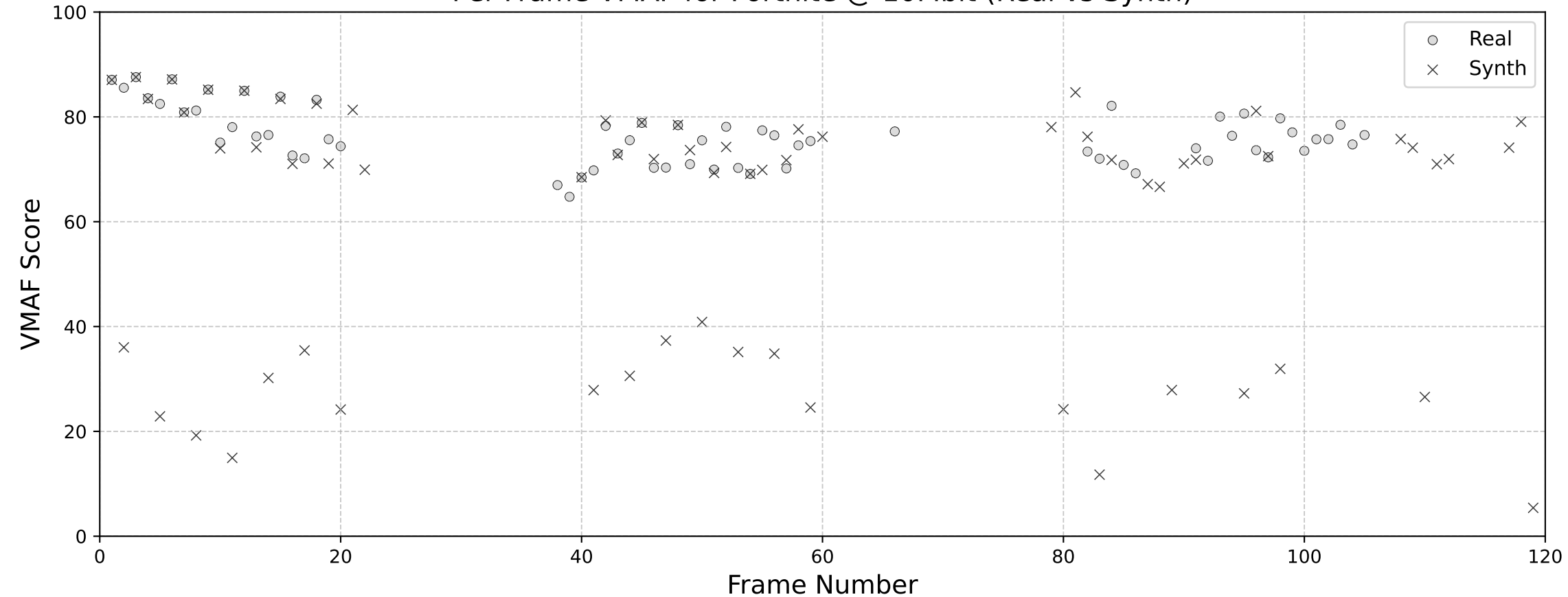
Per-Frame VMAF for Fortnite @ 10Mbit (Real vs Synth)
