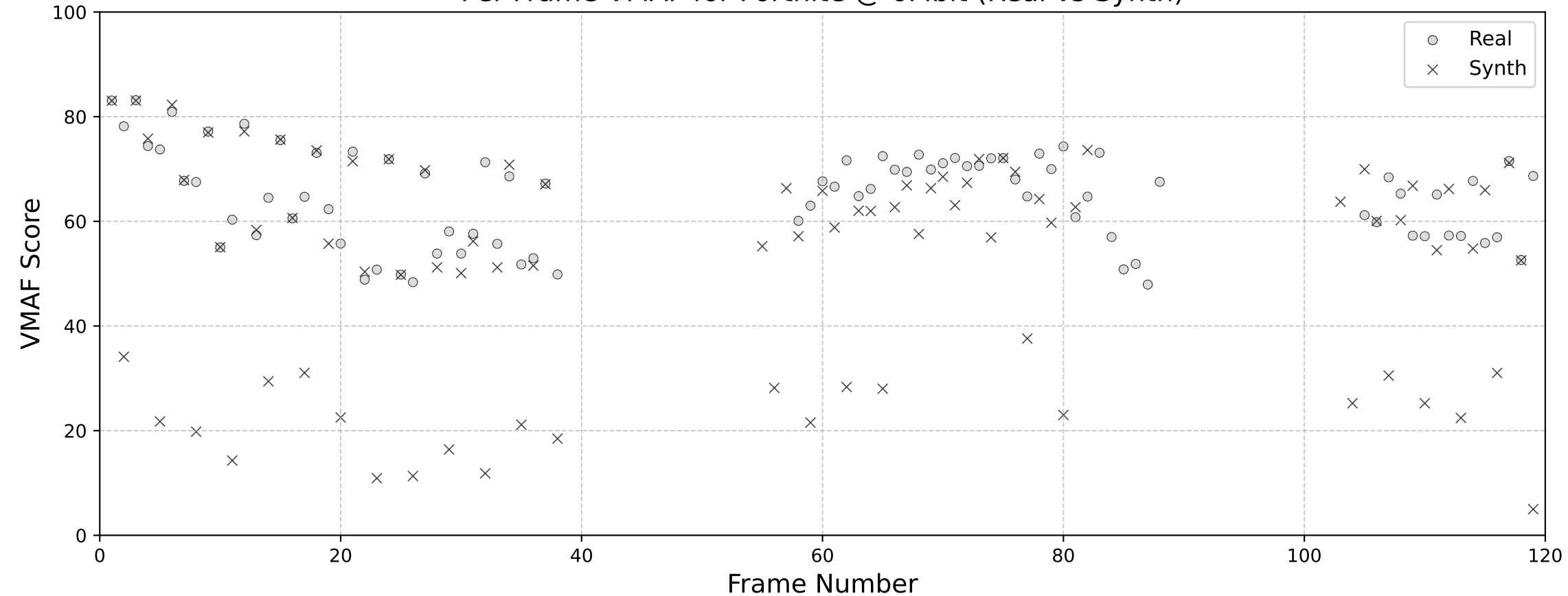
Per-Frame VMAF for Fortnite @ 6Mbit (Real vs Synth)
