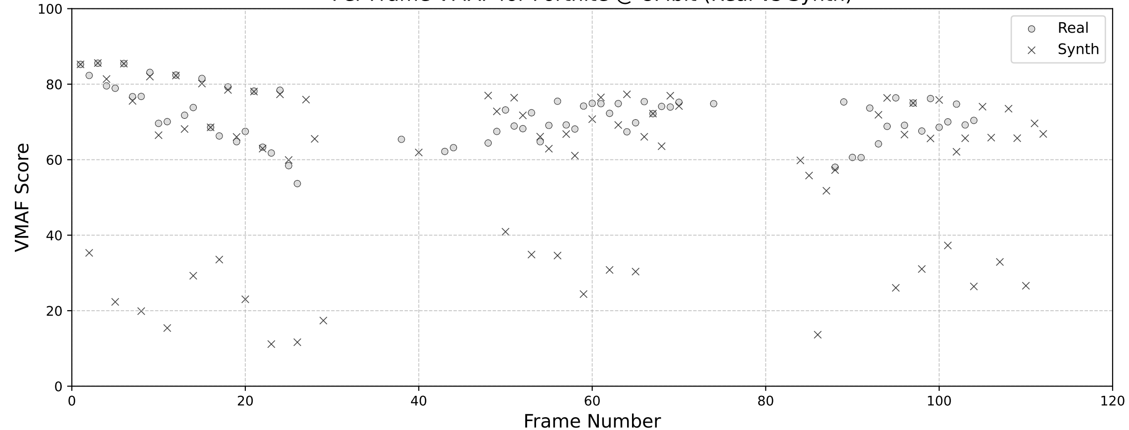
Per-Frame VMAF for Fortnite @ 8Mbit (Real vs Synth)
