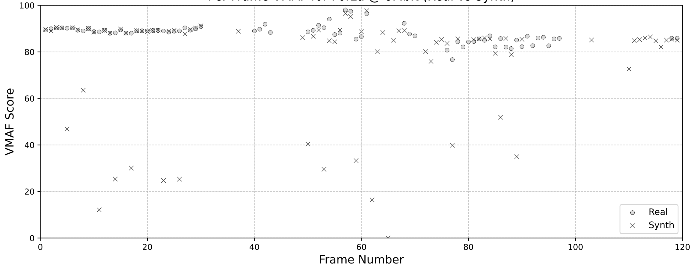
Per-Frame VMAF for Forza @ 8Mbit (Real vs Synth)
