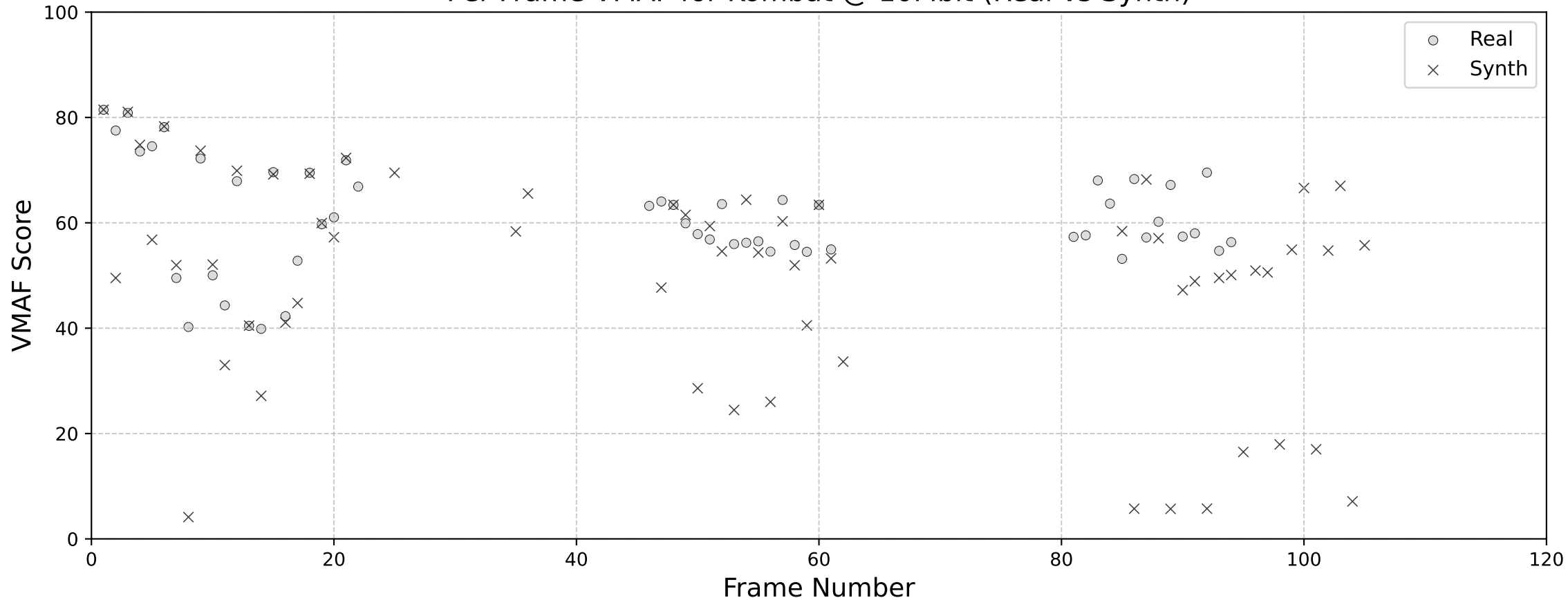
Per-Frame VMAF for Kombat @ 10Mbit (Real vs Synth)
