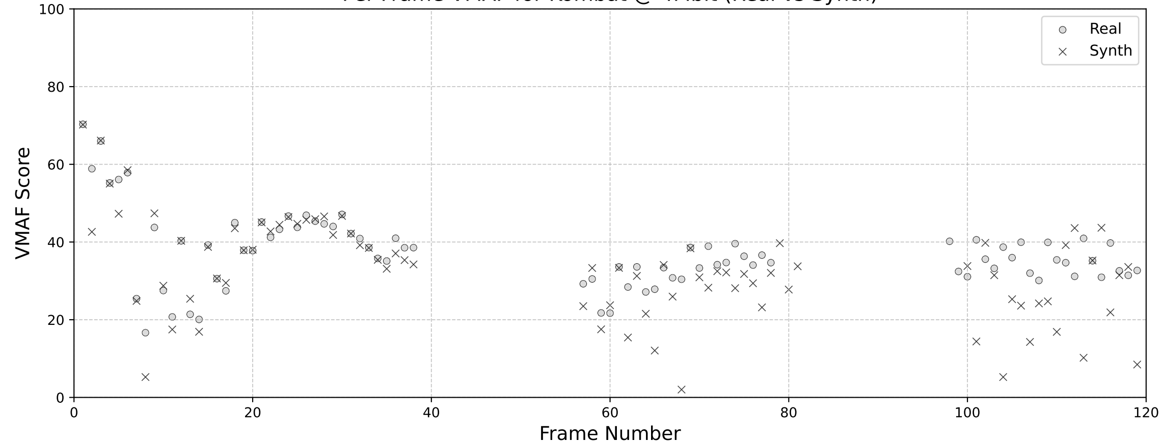
Per-Frame VMAF for Kombat @ 4Mbit (Real vs Synth)
