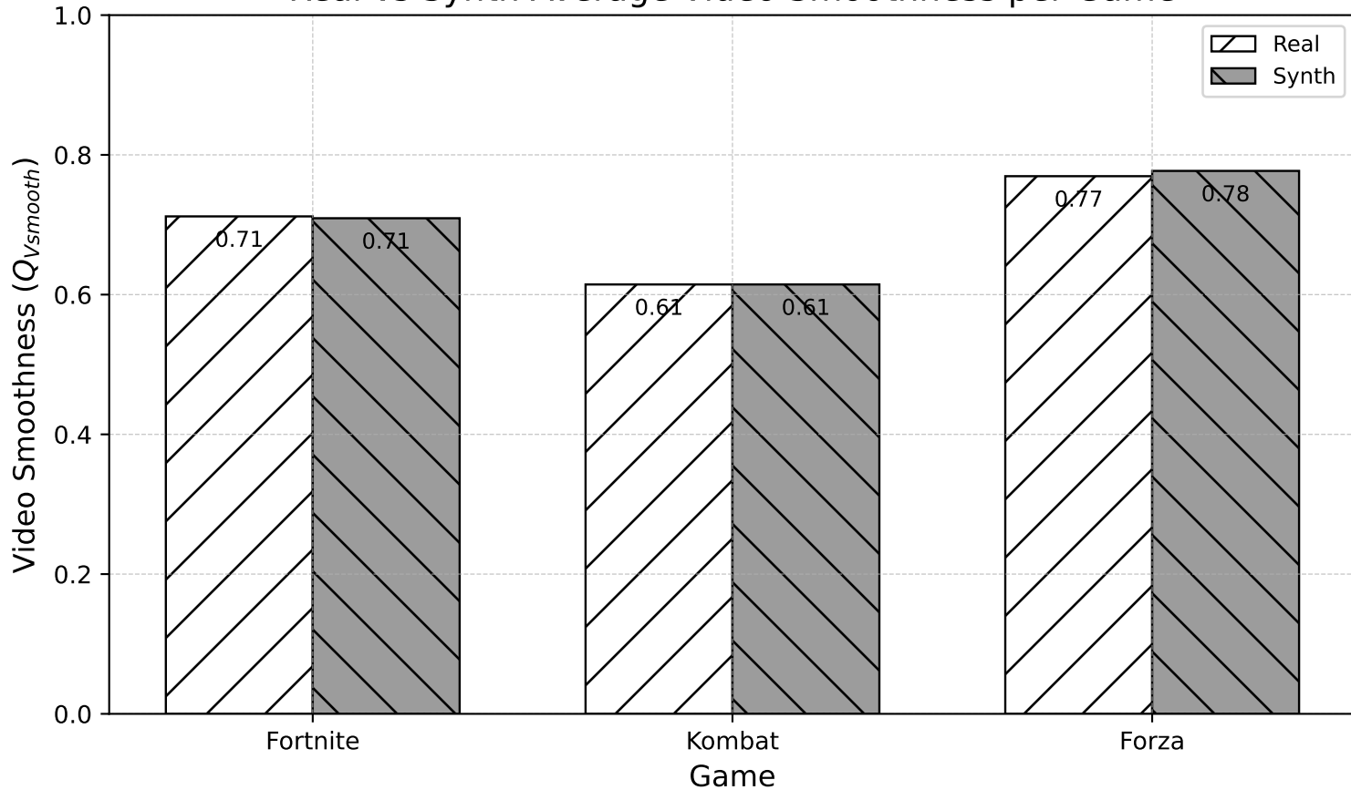
Real vs Synth Average Video Smoothness per Game
