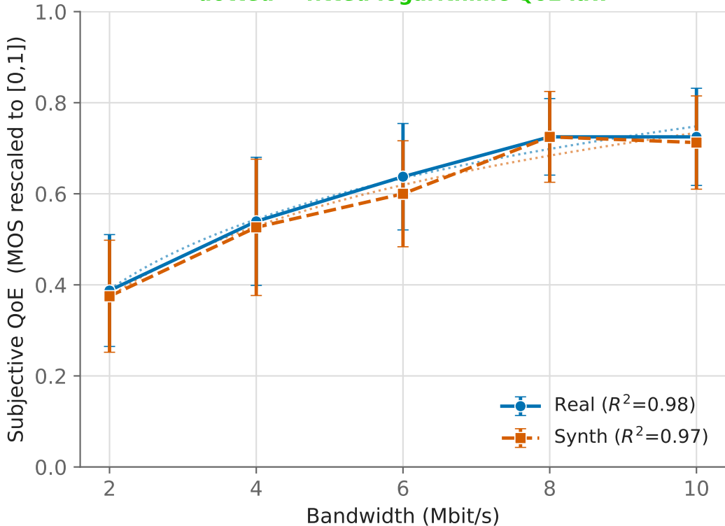
Forza — subjective QoE vs bandwidth (real vs synthetic) dotted = fitted logarithmic QoE law
