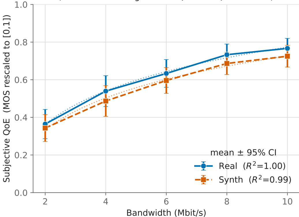
Subjective QoE vs bandwidth — real vs synthetic (dotted = fitted logarithmic QoE law Q = a \ln b + c )
