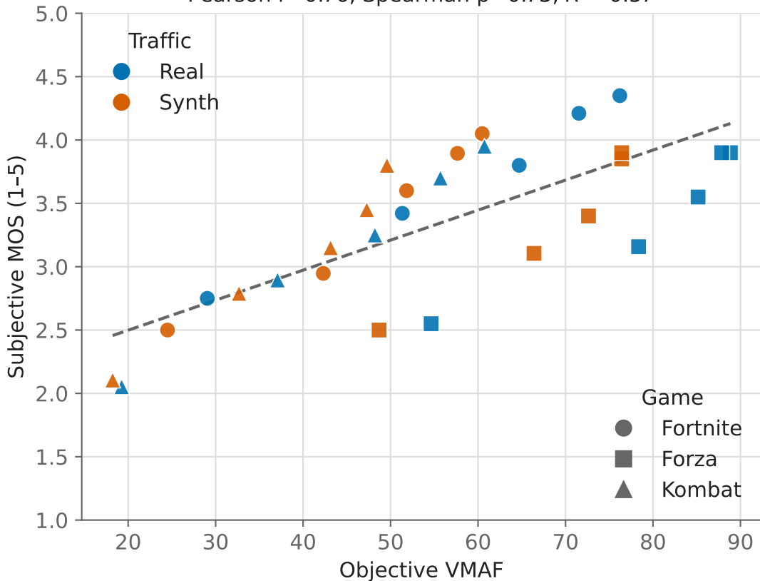
Objective VMAF vs subjective MOS Pearson r=0.76 , Spearman \rho=0.73 , R^2=0.57
