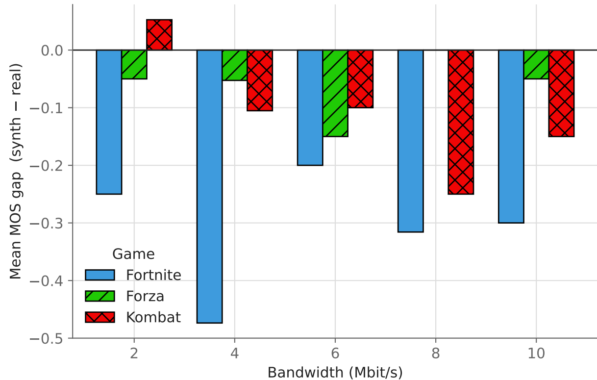
Synthetic-real MOS deviation per condition (near zero \rightarrow synthetic preserves perceived quality)
