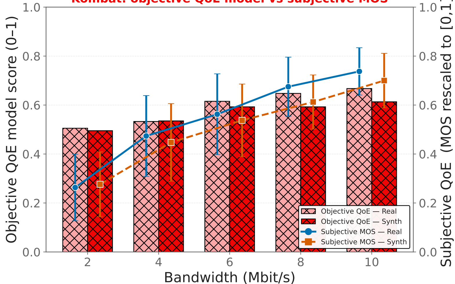
Kombat: objective QoE model vs subjective MOS
