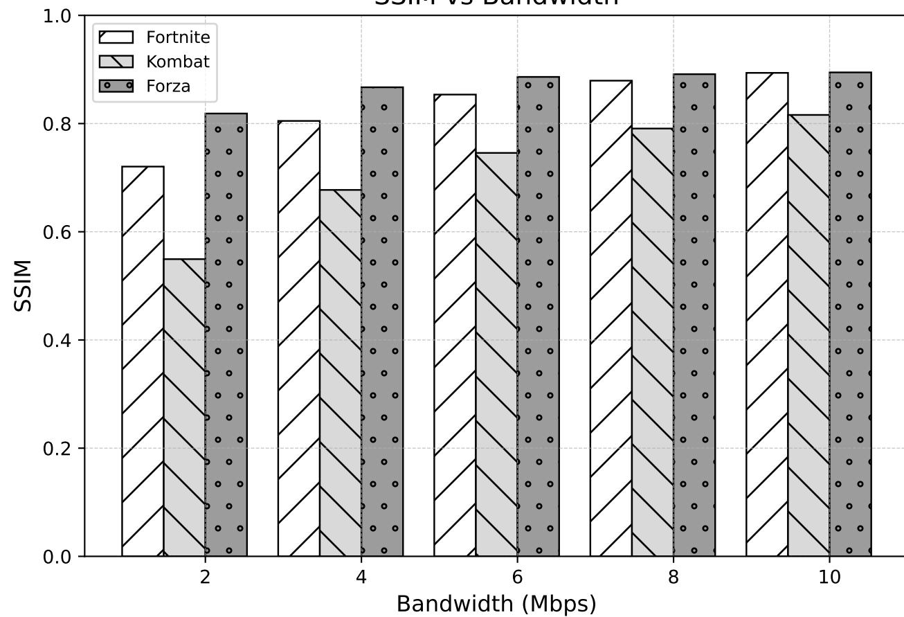
SSIM vs Bandwidth
