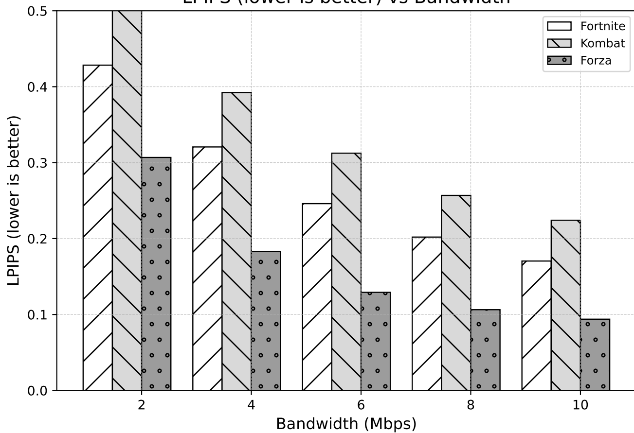
LPIPS (lower is better) vs Bandwidth
