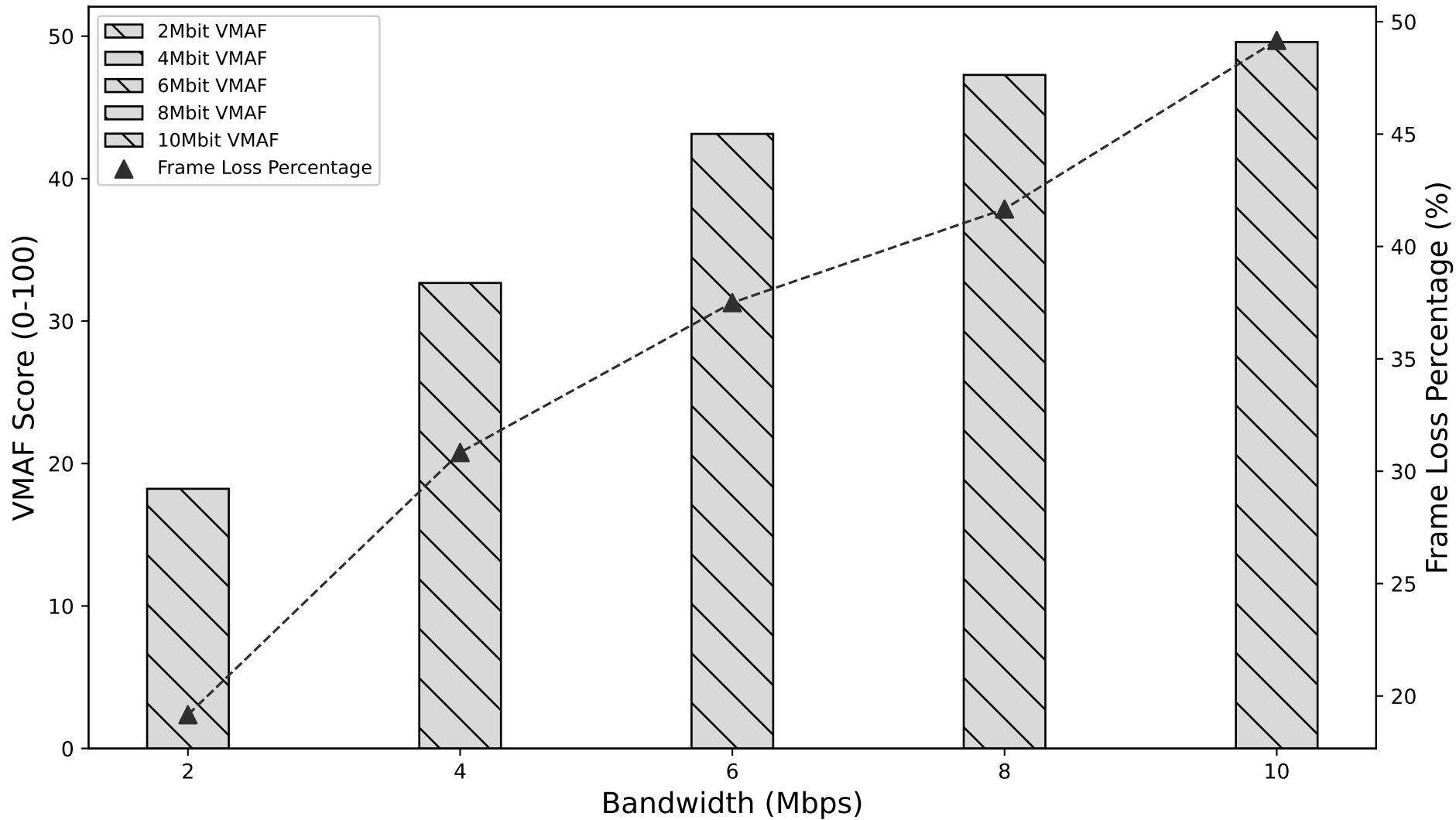
VMAF and Frame Loss vs. Bandwidth for Kombat
