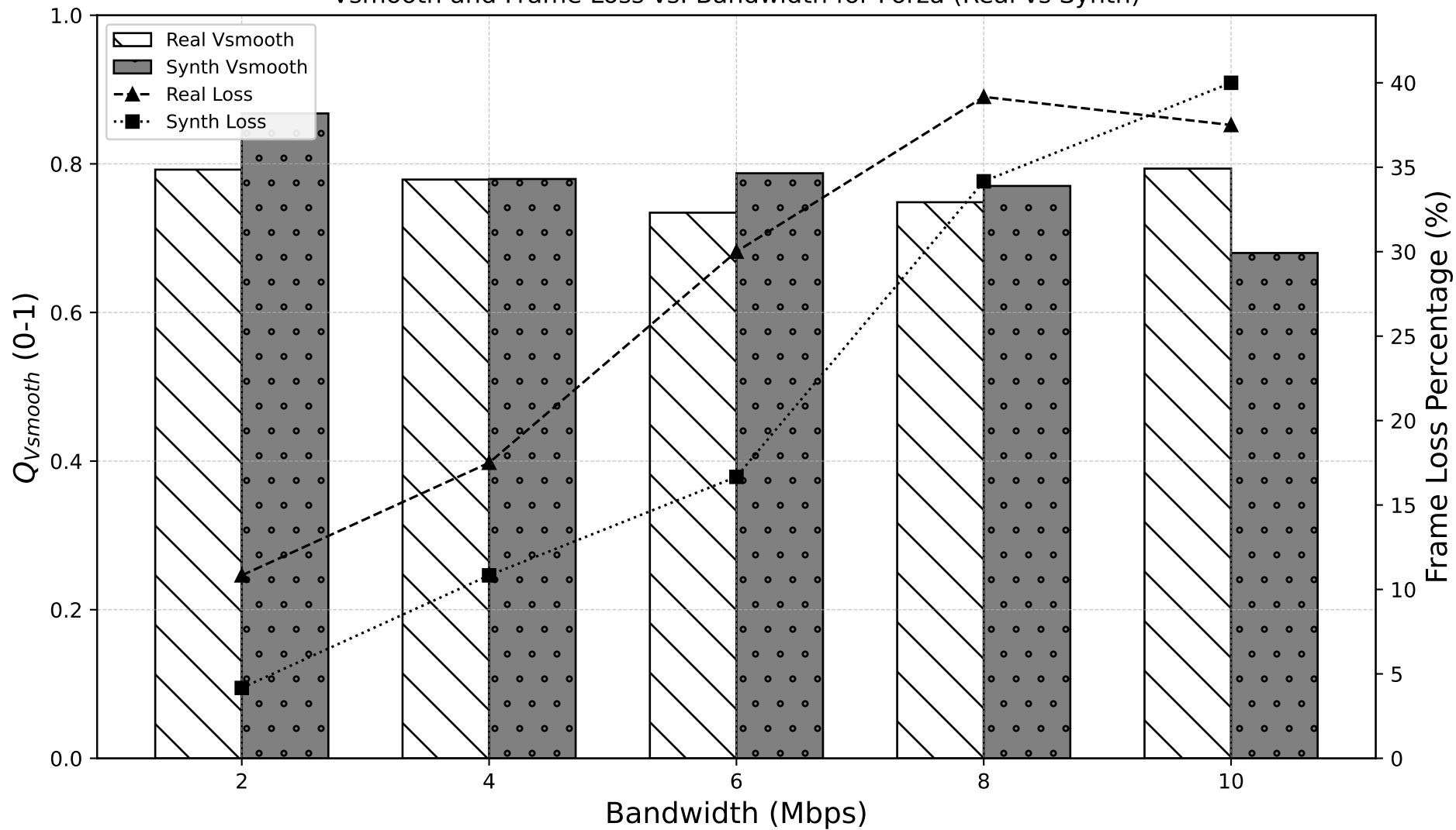
Vsmooth and Frame Loss vs. Bandwidth for Forza (Real vs Synth)
