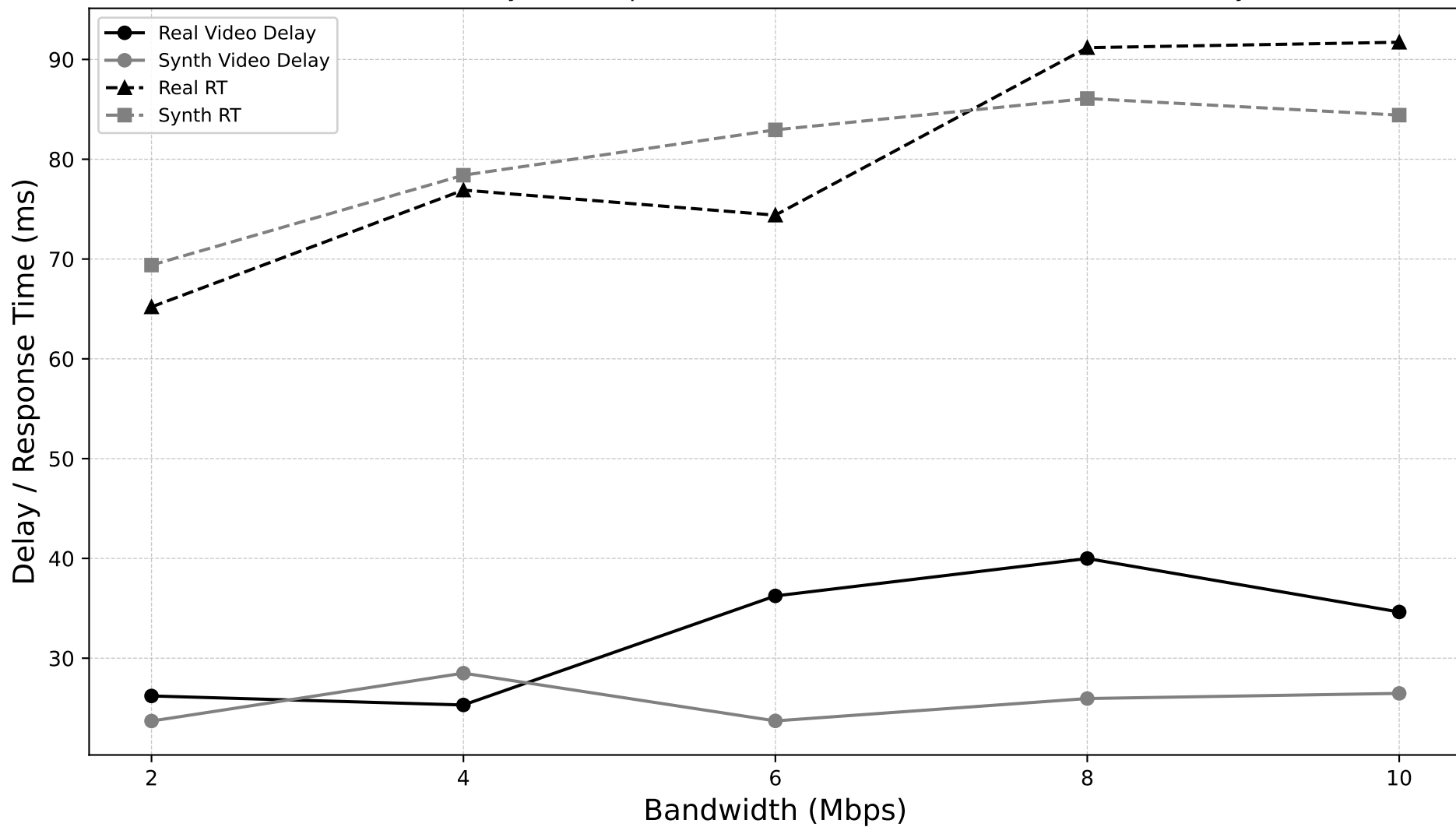
Downlink Video Delay and Response Time vs. Bandwidth for Fortnite (Real vs Synth)
