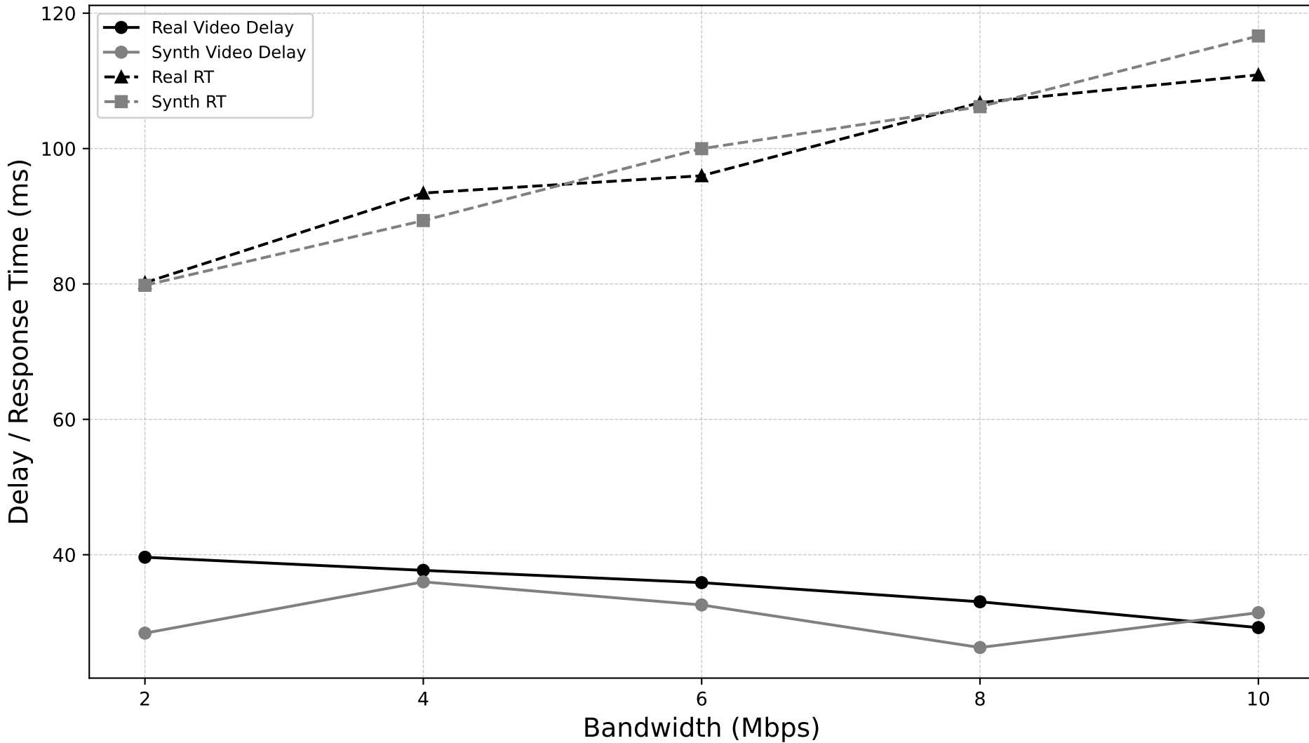
Downlink Video Delay and Response Time vs. Bandwidth for Kombat (Real vs Synth)
