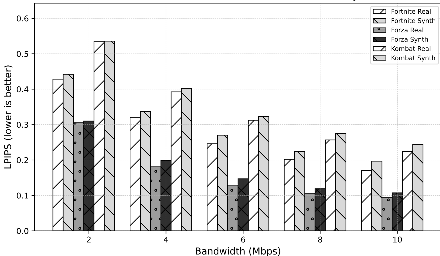
LPIPS (lower is better) vs Bandwidth (Real vs Synth)
