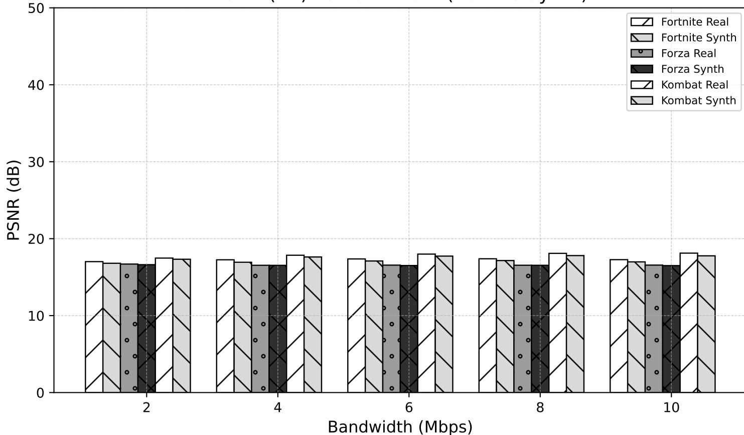
PSNR (dB) vs Bandwidth (Real vs Synth)
