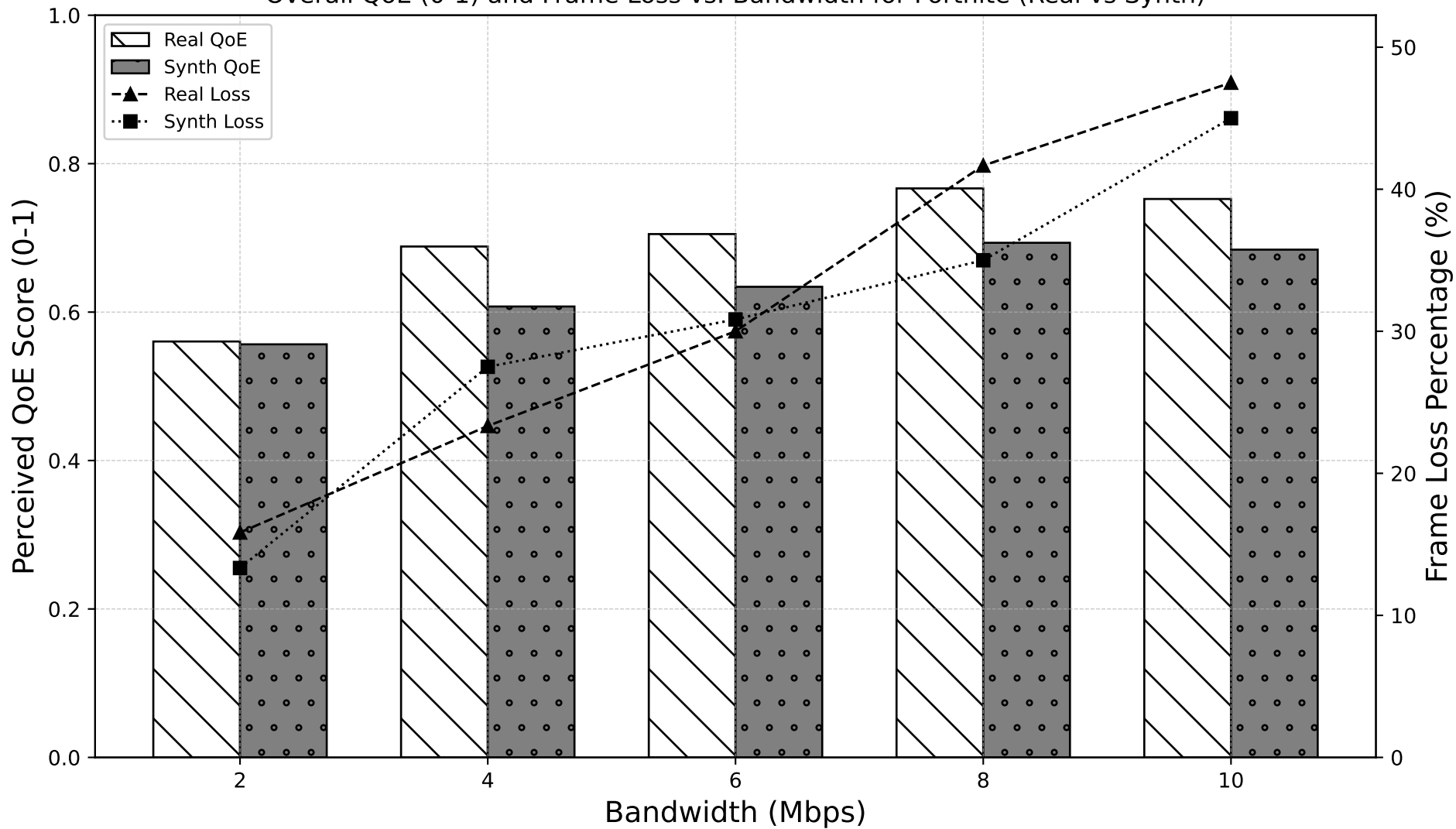
Overall QoE (0-1) and Frame Loss vs. Bandwidth for Fortnite (Real vs Synth)
