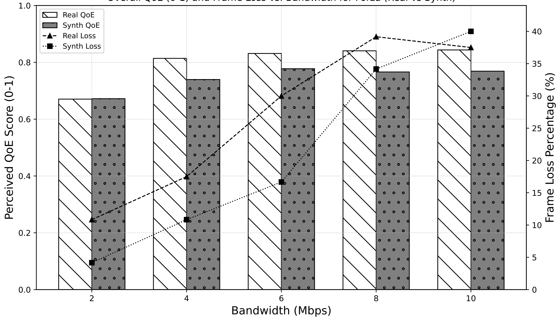
Overall QoE (0-1) and Frame Loss vs. Bandwidth for Forza (Real vs Synth)
