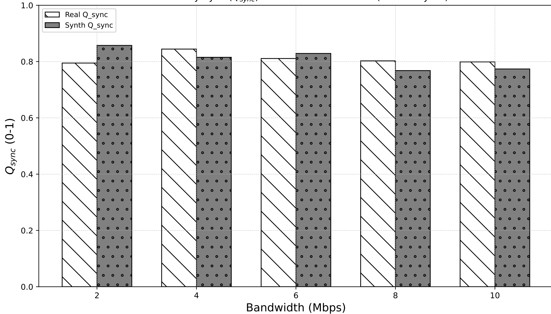
Interactivity Sync ( Q_{sync} ) vs. Bandwidth for Forza (Real vs Synth)
