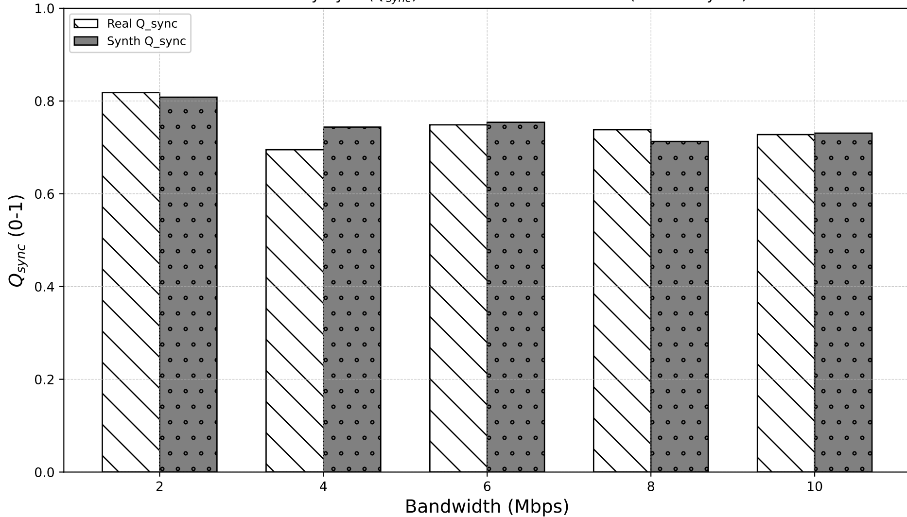
Interactivity Sync ( Q_{sync} ) vs. Bandwidth for Kombat (Real vs Synth)
