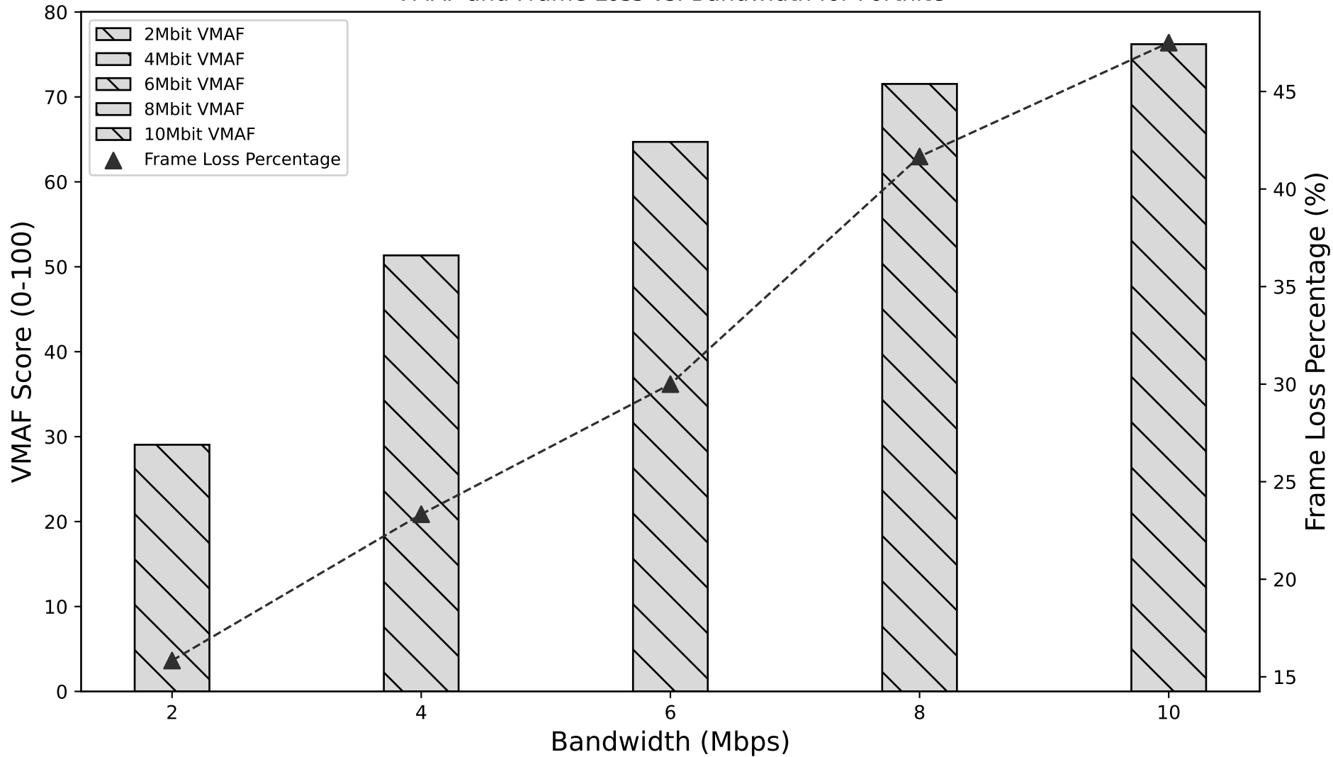
VMAF and Frame Loss vs. Bandwidth for Fortnite
