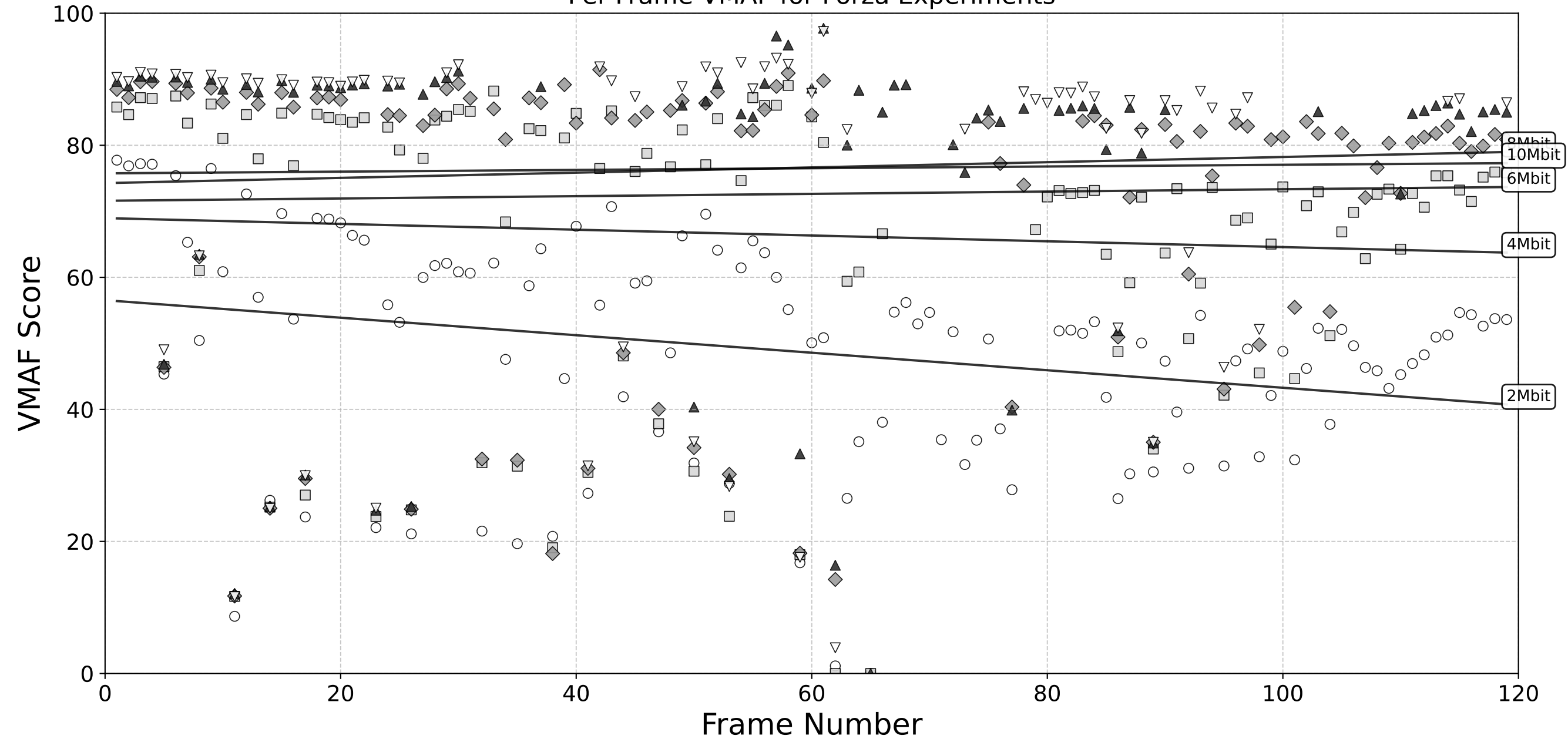
Per-Frame VMAF for Forza Experiments
