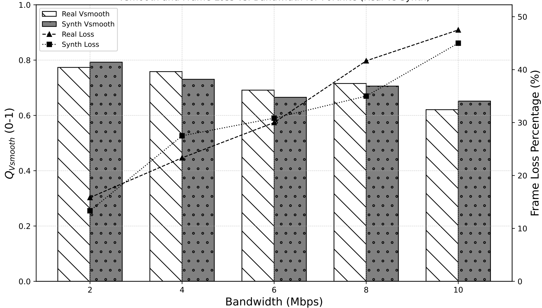
Vsmooth and Frame Loss vs. Bandwidth for Fortnite (Real vs Synth)
