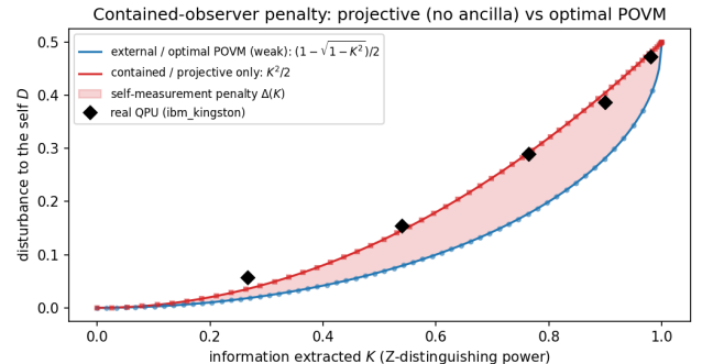
Figure 2: The projective frontier K^2/2 (contained, no ancilla) lies strictly above the optimal POVM bound; black markers are real-QPU measurements.
