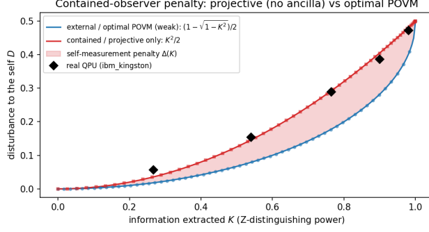
Figure 2: The projective frontier K^2/2 (contained, no ancilla) lies strictly above the optimal POVM bound; black markers are real-QPU measurements.
