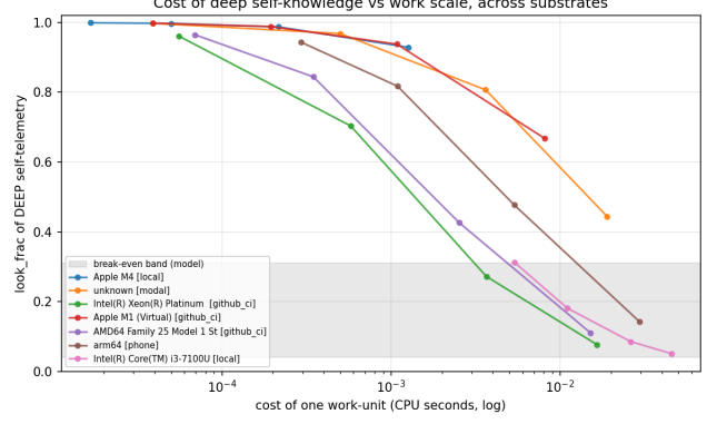
Figure 3: Cost of deep self-knowledge vs. work scale across substrates; the look-cost is denominator-free and the conclusion robust across the sweep.
