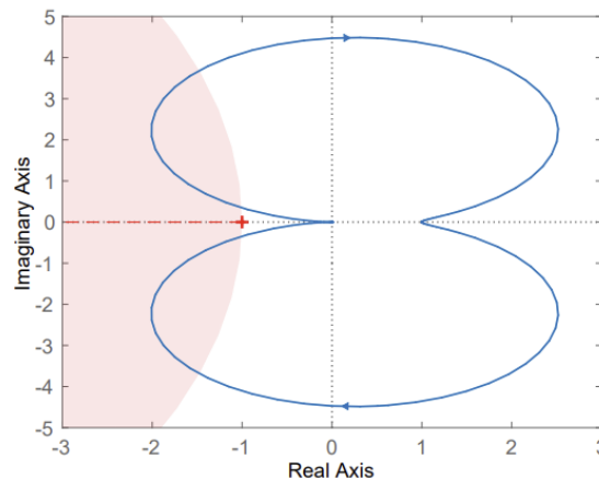
Figure 18: [Solid line] Nyquist plot of L . [Dashed line] plot of N(u) as the gain varies within the segment [\frac{-1}{k_1}, \frac{-1}{k_2}] . [Shaded circle] Circle with diameter [\frac{1}{k_1}, \frac{1}{k_2}] .
