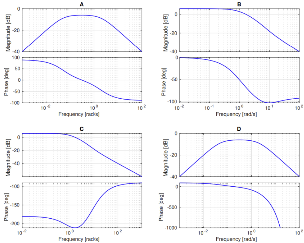
Figure 8: Bode plots of G_1 , G_2 , G_3 and G_4 in random order.
