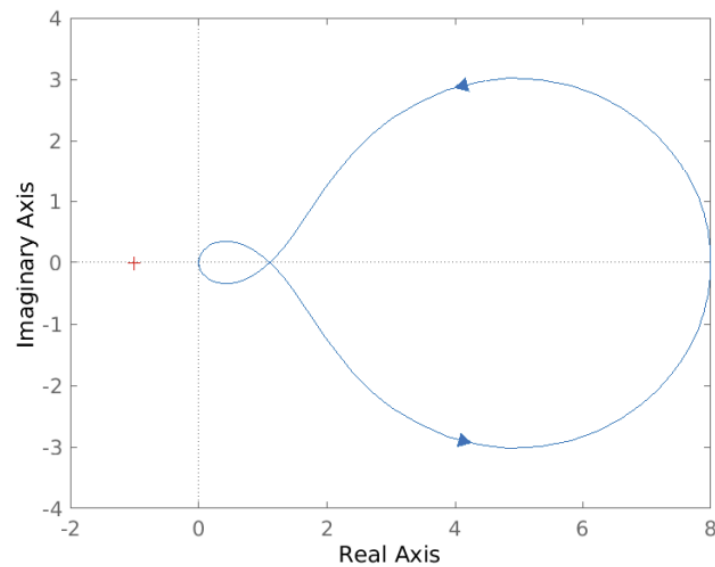
Figure 10: Nyquist plot of L(s) .
