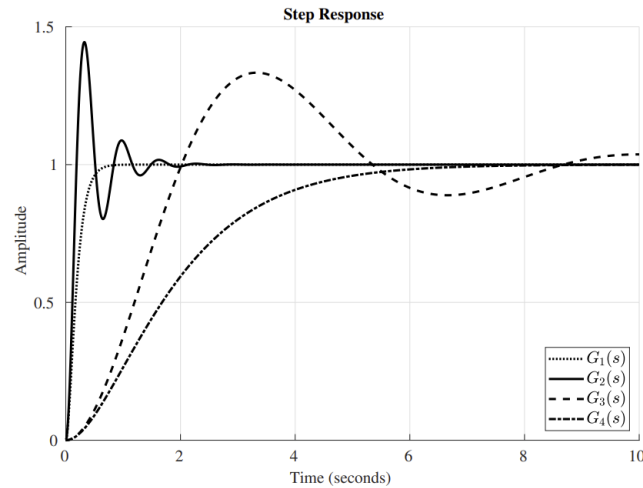
Figure 11: Step responses of second order linear-time invariant systems G_i(s) , i = 1, 2, 3, 4 .
