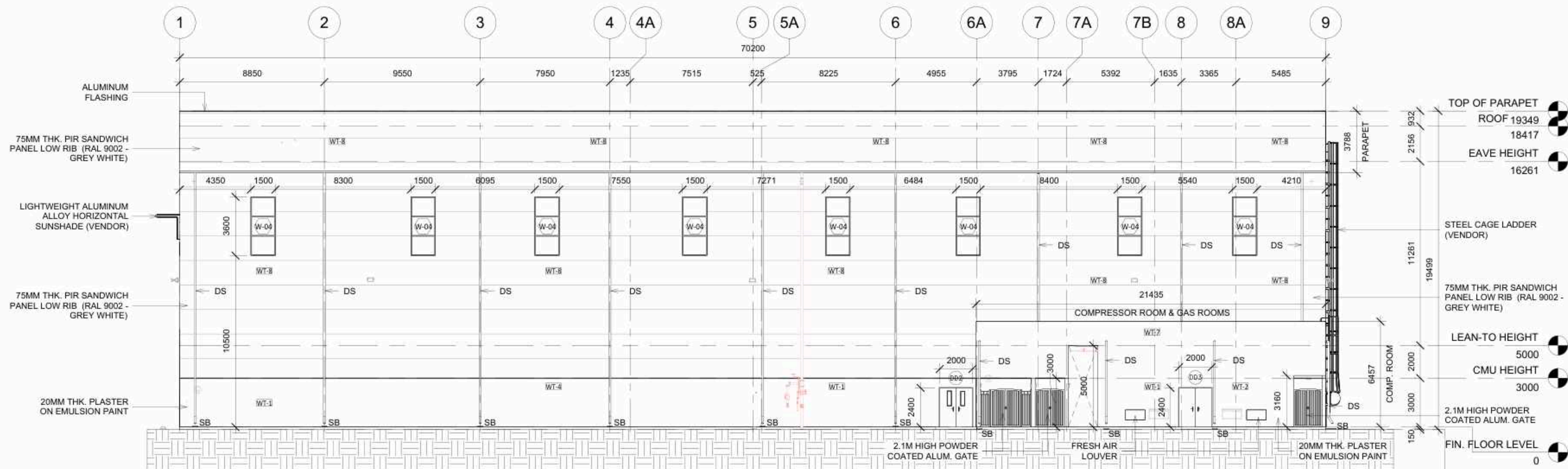
2 WEST ELEVATION 1 : 150
