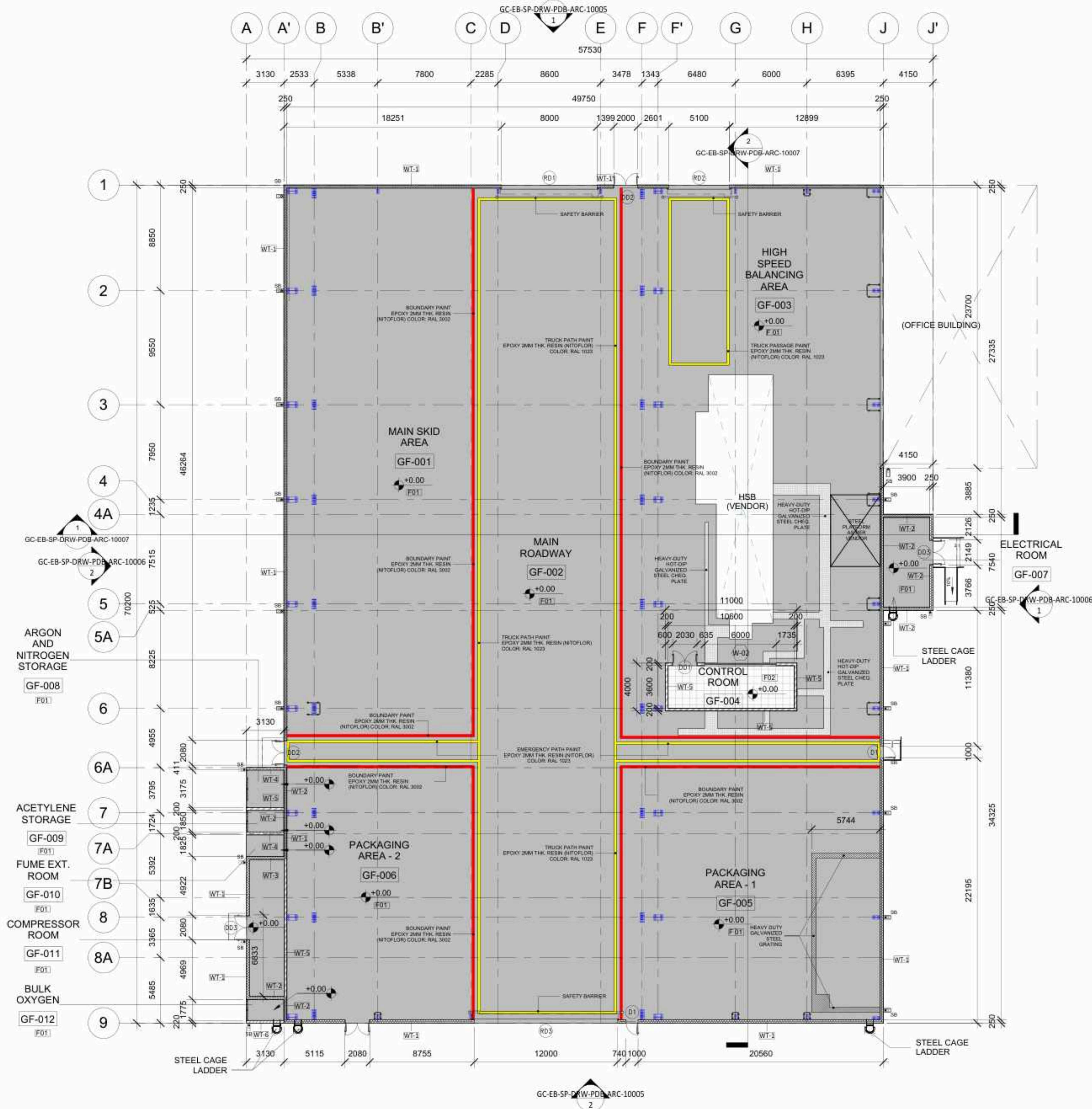
1 GROUND FLOOR PLAN 1 : 200
