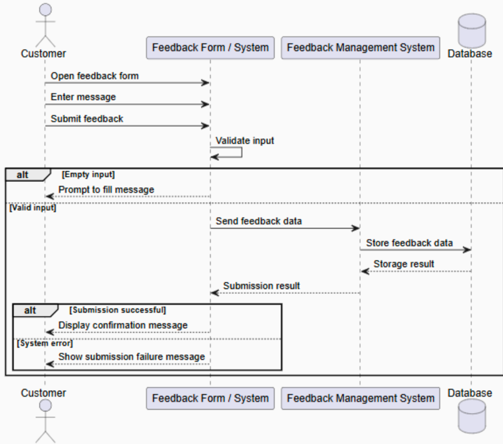
UC17 - Submit Feedback or Complaint Sequence Diagram
