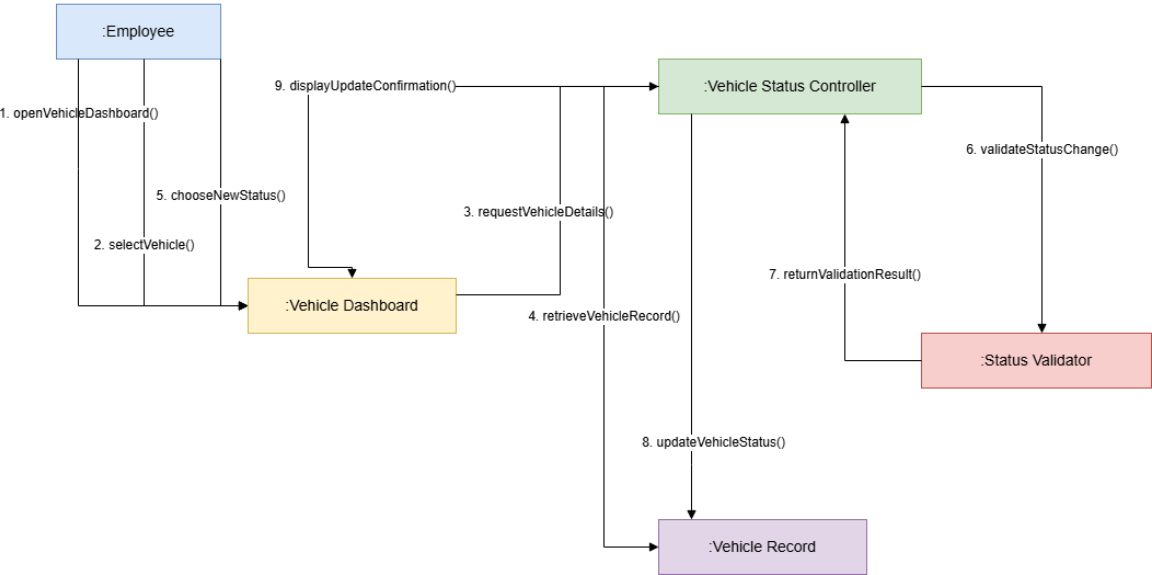
UC23 - Manage Vehicle Status Communication Diagram
