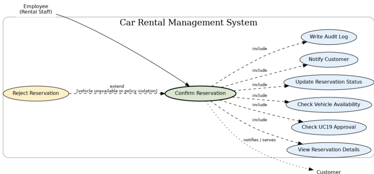
UC20 - Confirm Reservation Use Case Diagram
