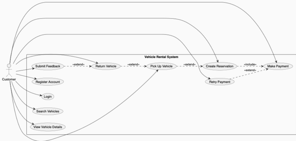
Use Case Diagram - Customer
