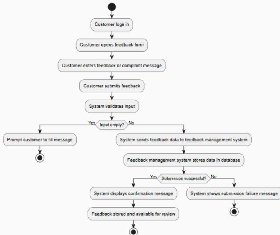
UC17 - Submit Feedback or Complaint Activity Diagram
