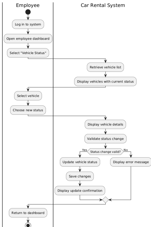
UC23 - Manage Vehicle Status Activity Diagram
