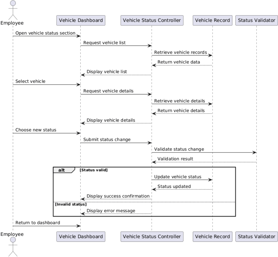
UC23 - Manage Vehicle Status Sequence Diagram
