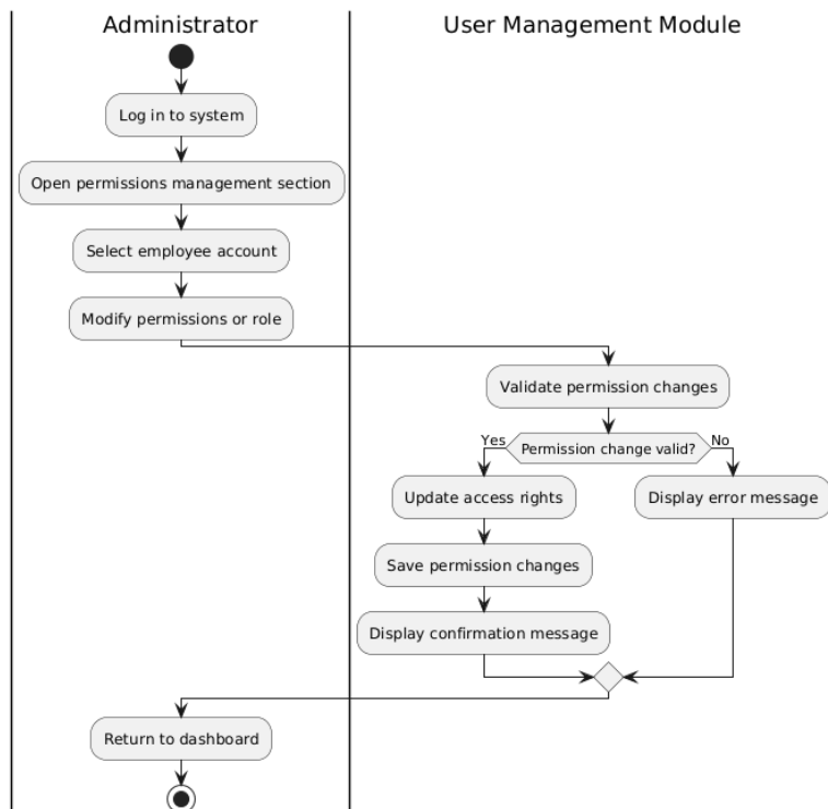
UC30 - Manage User Permissions Activity Diagram
