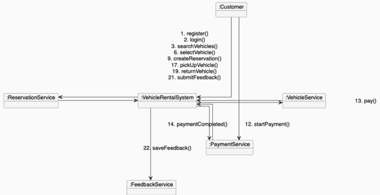
Collaboration Diagram - Customer Vehicle Rental Process
