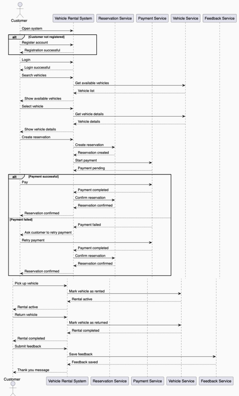
Sequence Diagram - Customer Vehicle Rental Process
