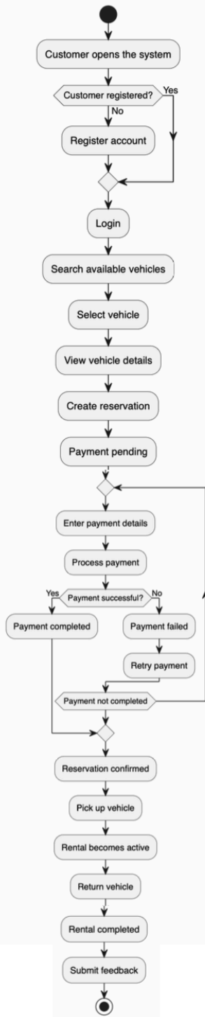
Activity Diagram - Customer Vehicle Rental Process
