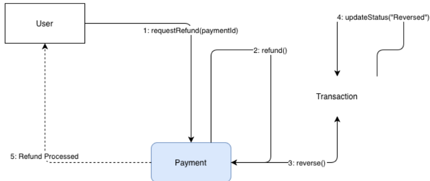
-DIAGRAM 2: Refund Payment
