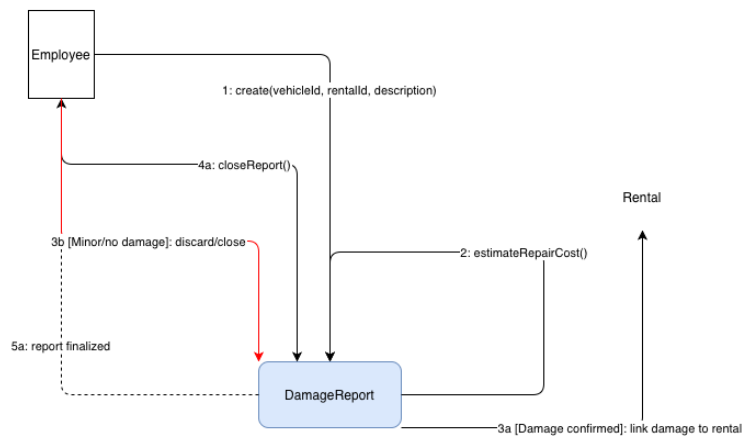
-DIAGRAM 19: Damage Reporting Process
