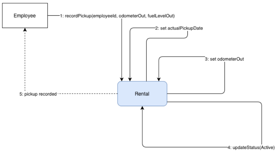
-DIAGRAM 16: Record Vehicle Pickup
