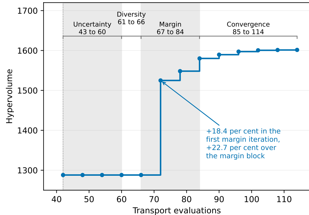
(a) Hypervolume by acquisition revision
