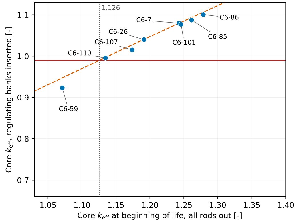
(a) Four regulating banks
