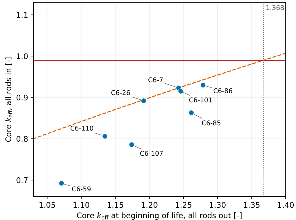
(b) All rods in
