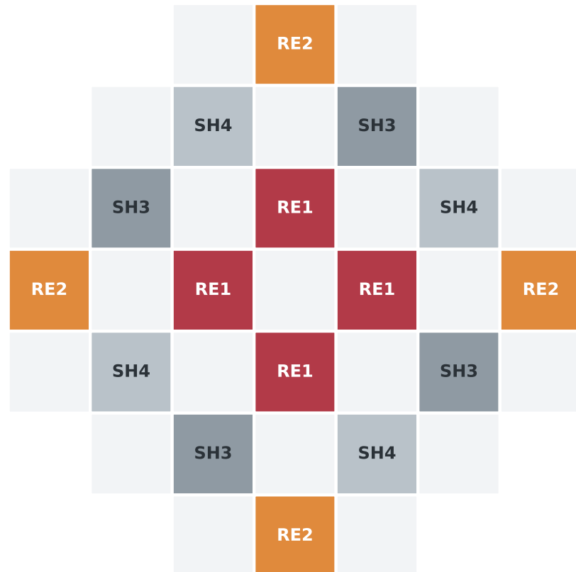
(b) NuScale-like reference, 37 assemblies
