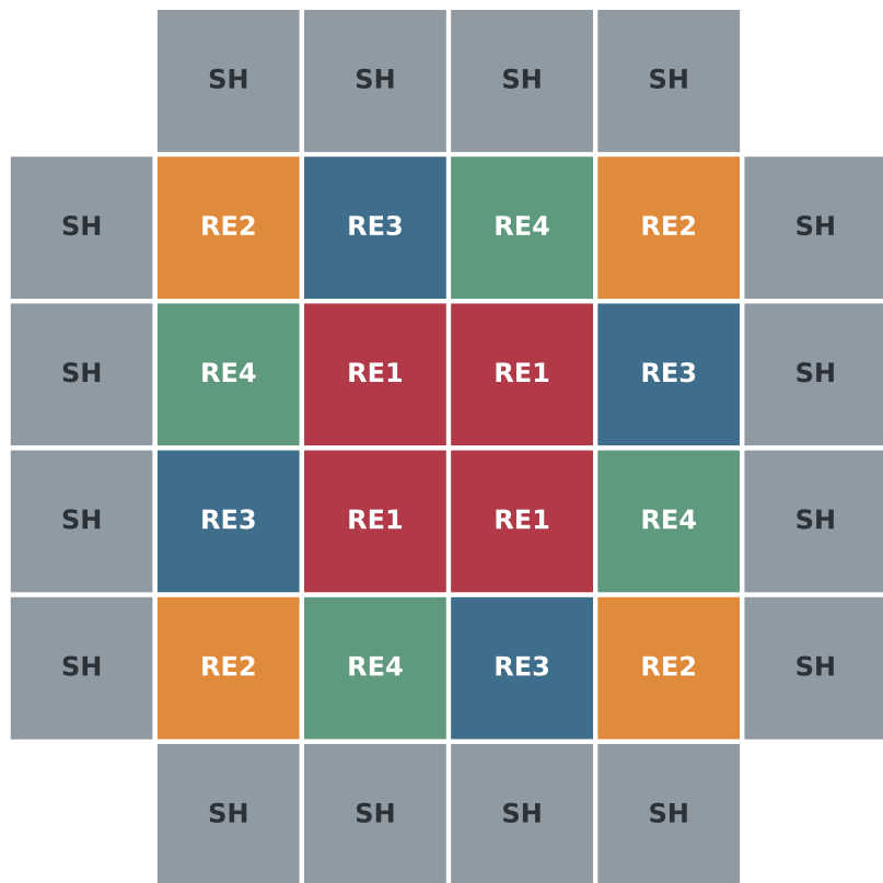
(a) This work, 32 assemblies
