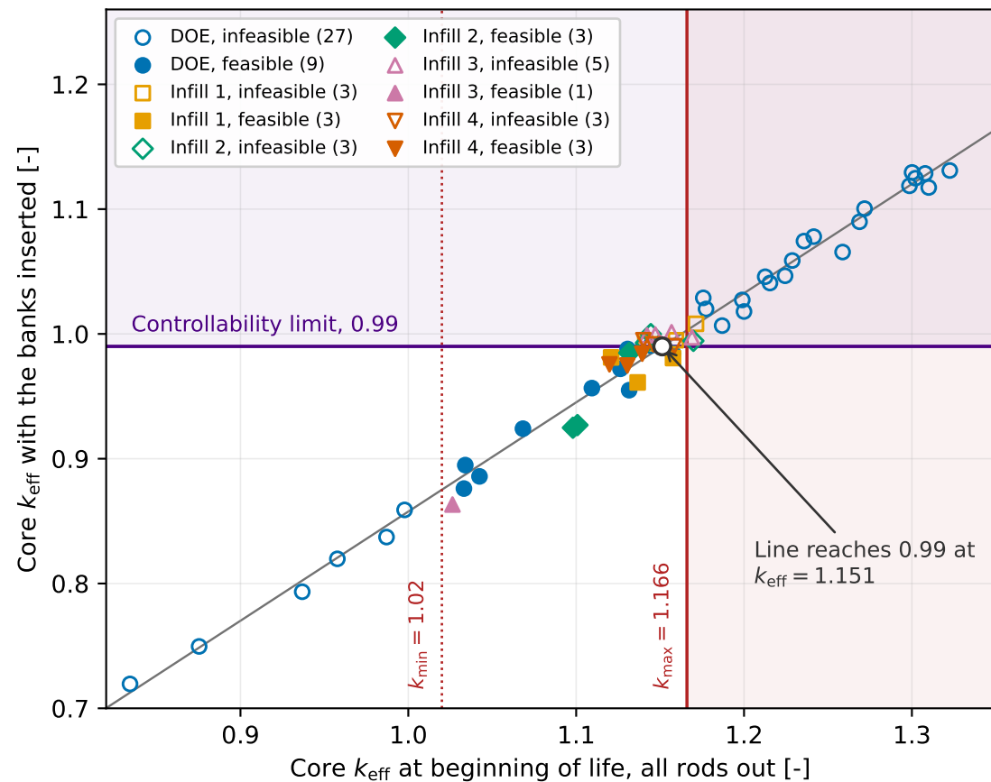
(a) Four banks, RE1 to RE4, sixteen assemblies: the constrained state
