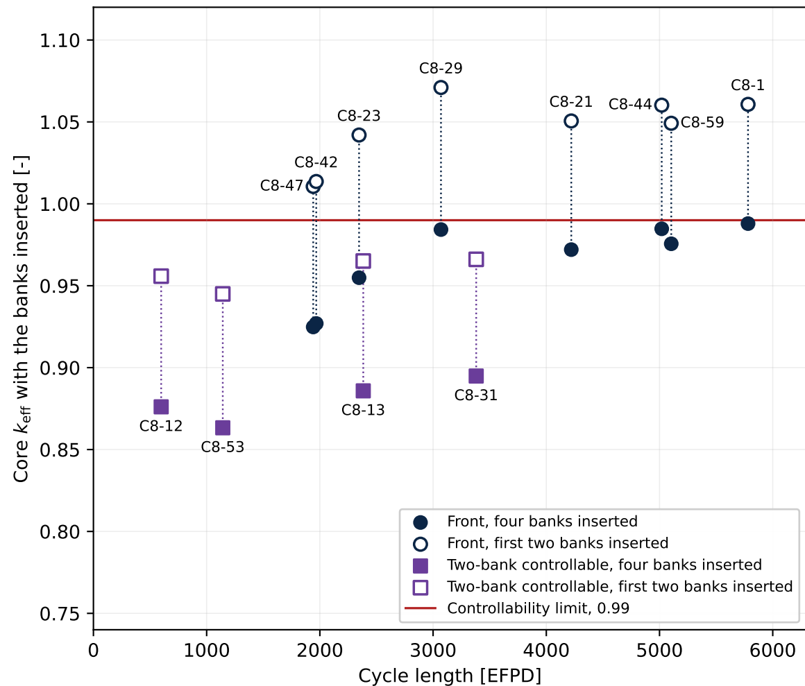
(a) Controllability margin
