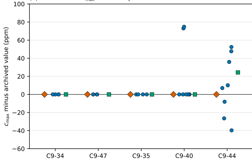
(b) Critical boron c_{\max} of each depletion
