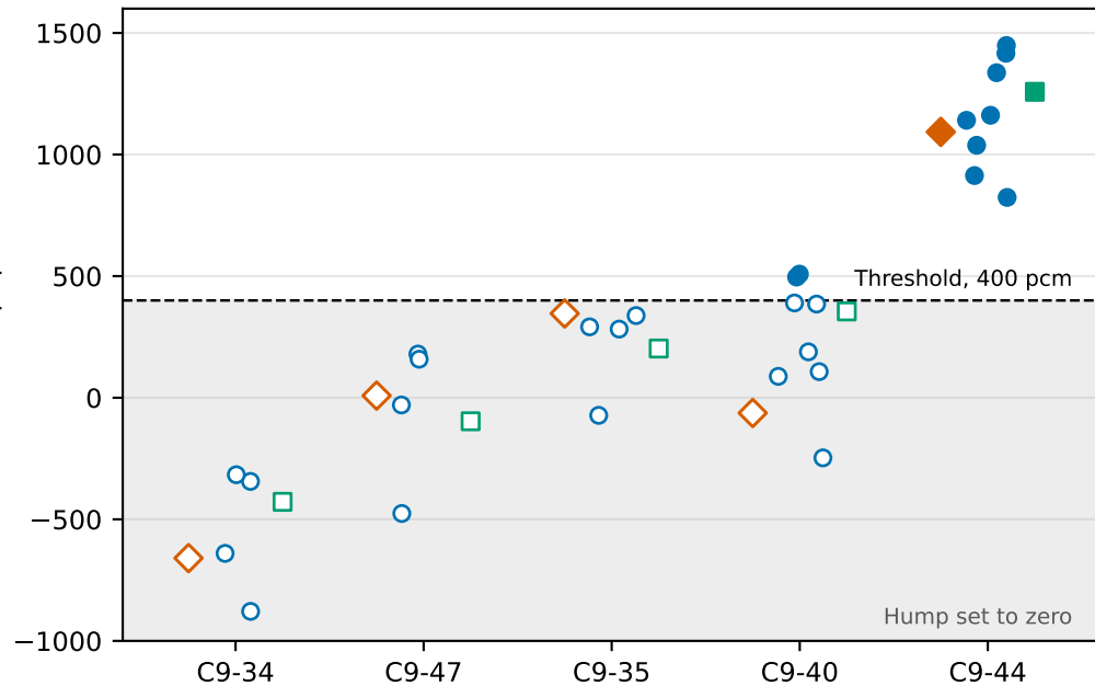
(a) Hump of each depletion against the threshold
