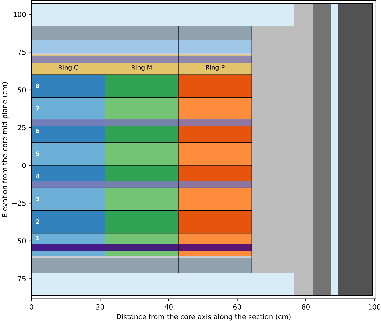
(b) Core, vertical half section: 8 depletion layers of 15 cm
