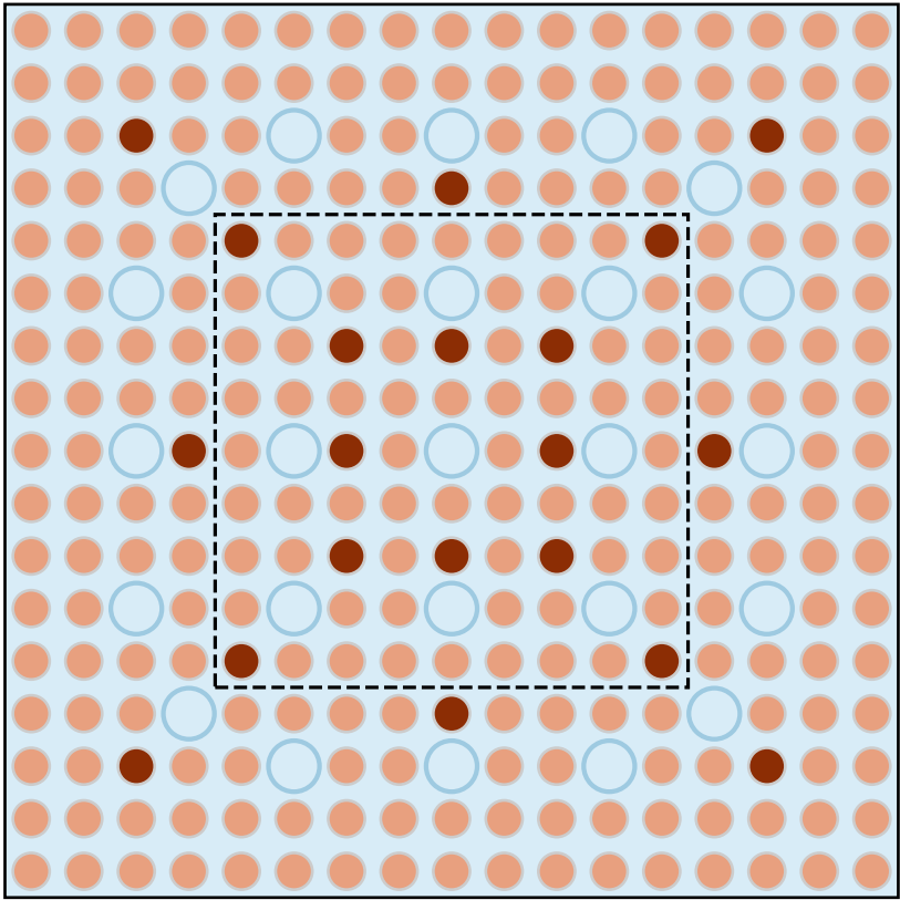
(a) Assembly of C9-47, radial section
