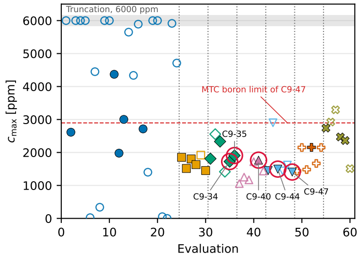
(b) Critical boron at the operating maximum
