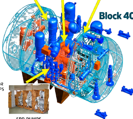
SRR PUMPS
