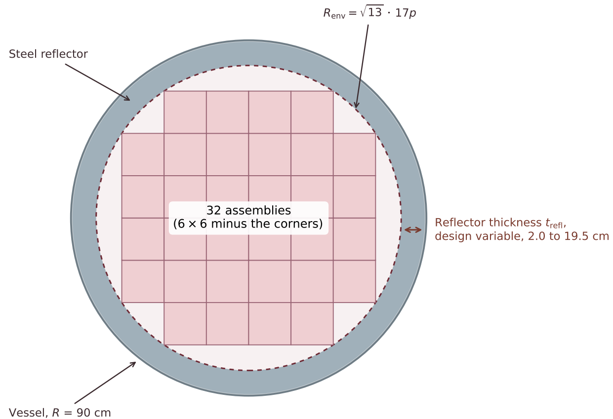
(b) The core plan view, drawn at p = 1.26 cm and t_{refl} = 12 cm
