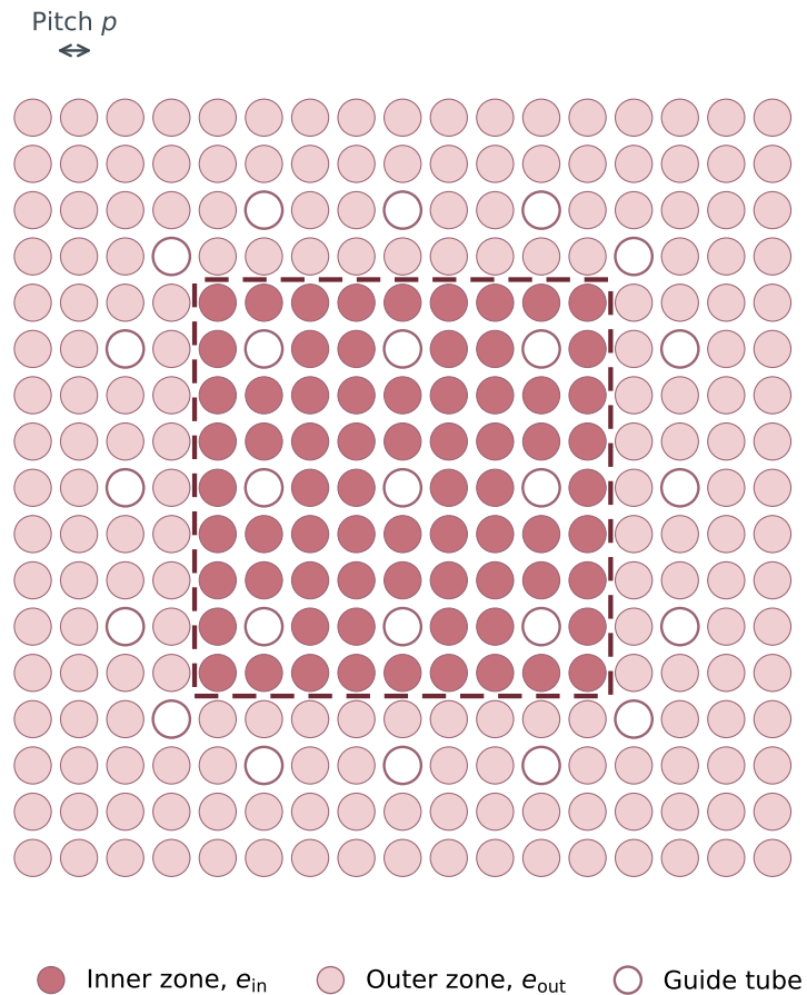
(a) The 17 \times 17 assembly
