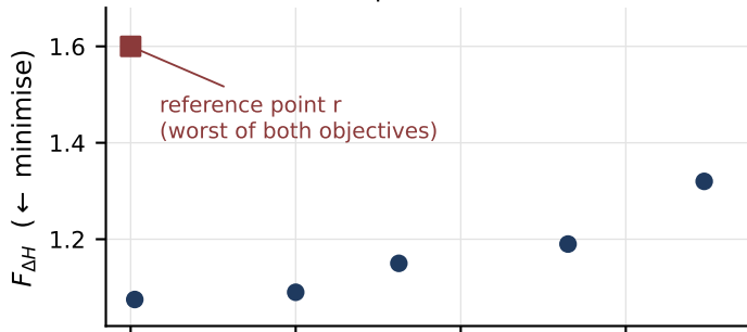
(a) fix the reference point once
