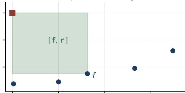
(b) one member spans one rectangle
