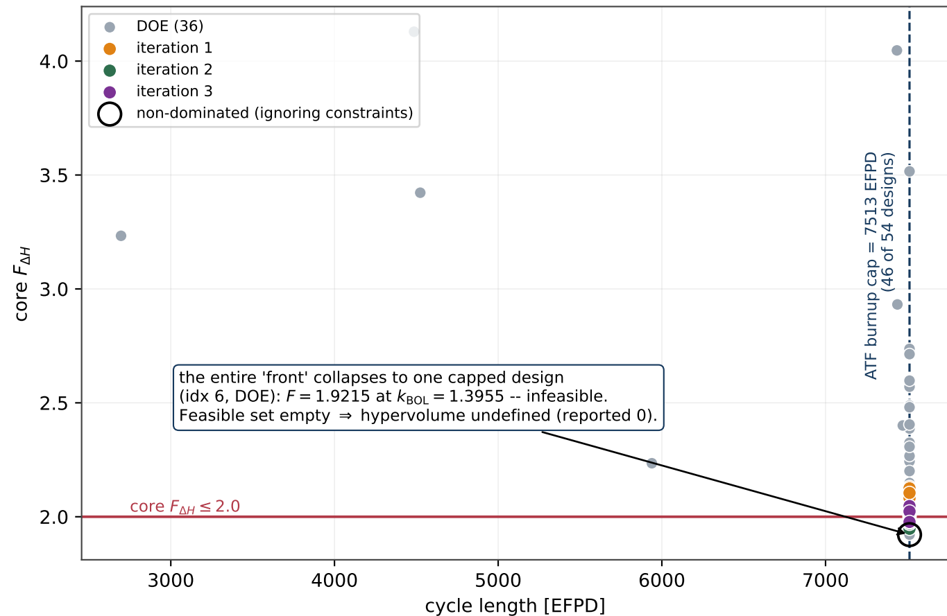
Campaign 4, objective plane: the burnup cap degenerates the trade-off
