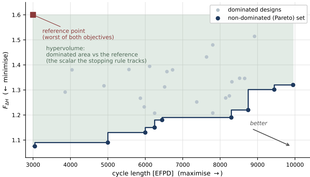
Dominance, the Pareto front, and hypervolume (synthetic data)
