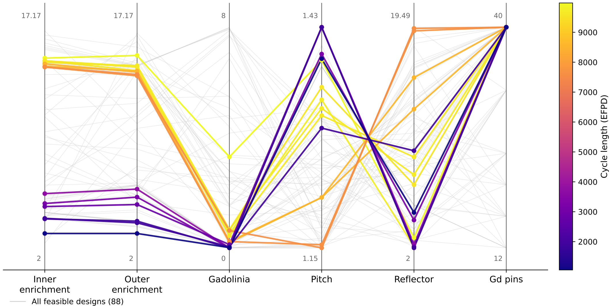
Campaign 6: the 15 Pareto-front designs across the six design variables
